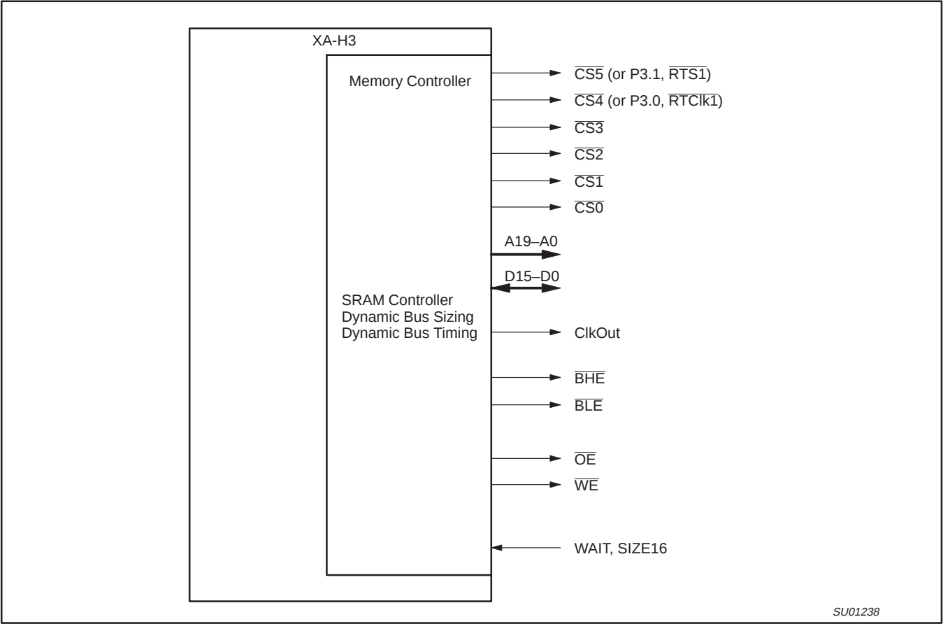
Figure 3. Memory Bus Interface Signal Pins
